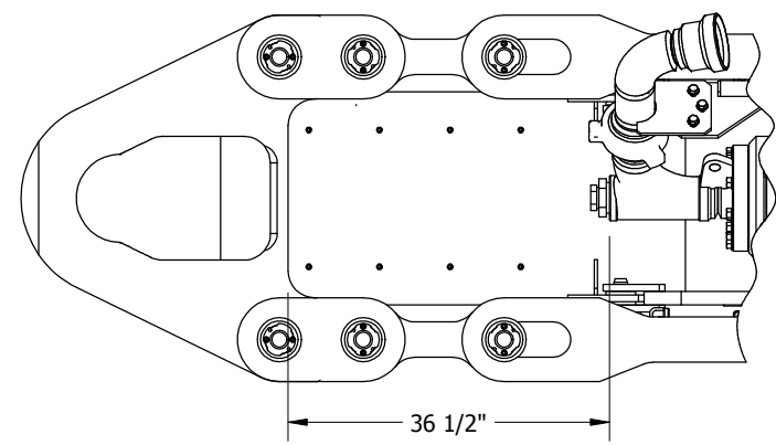
Optional Extension Links for Wireline Sheave
